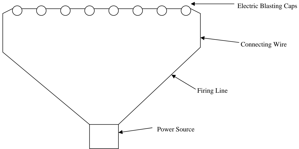
Diagram 3-2. Wiring Configurations
